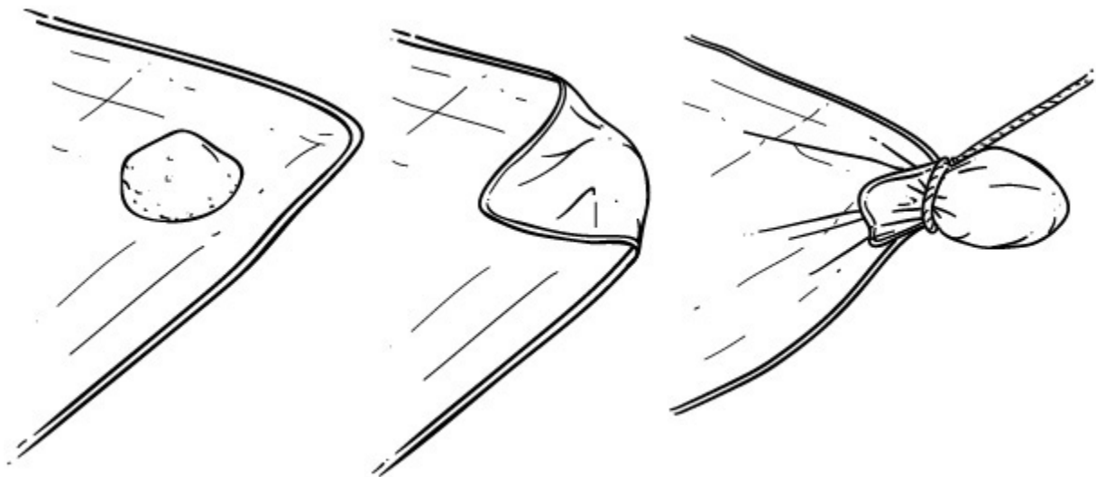
Tarp loop attachments with rocks
